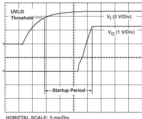
Figure 18. PTH08040W Startup
