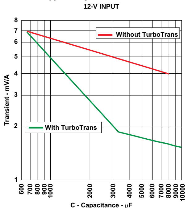
Figure 12. Capacitor Type B, 1000 < C(μF)×ESR(mΩ) ≤ 5000 (e.g. Polymer-Tantalum)
