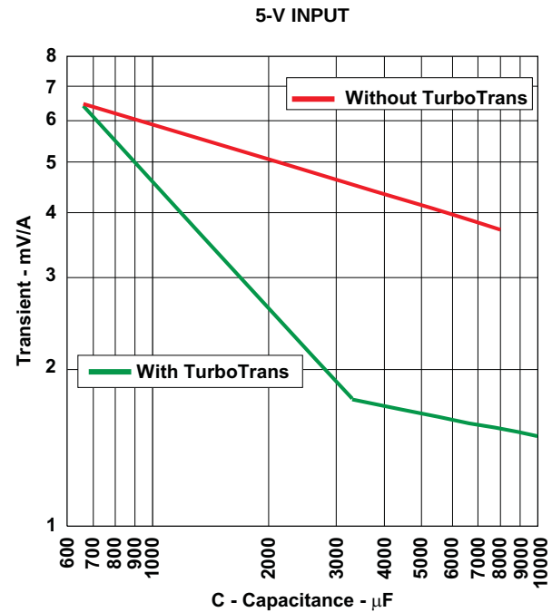
Figure 15. Capacitor Type C, 5000 < C(μF)×ESR(mΩ) ≤ 10,000(e.g. OS-CON)
