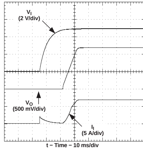
Figure 18. Power-Up Waveform
