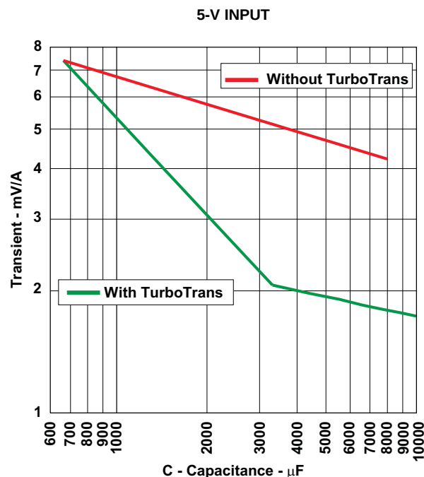
Figure 13. Capacitor Type B, 1000 < C(μF)×ESR(mΩ) ≤ 5000 (e.g. Polymer-Tantalum)
