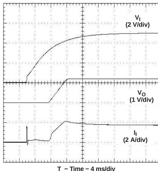
Figure 20. Power-Up Waveform
