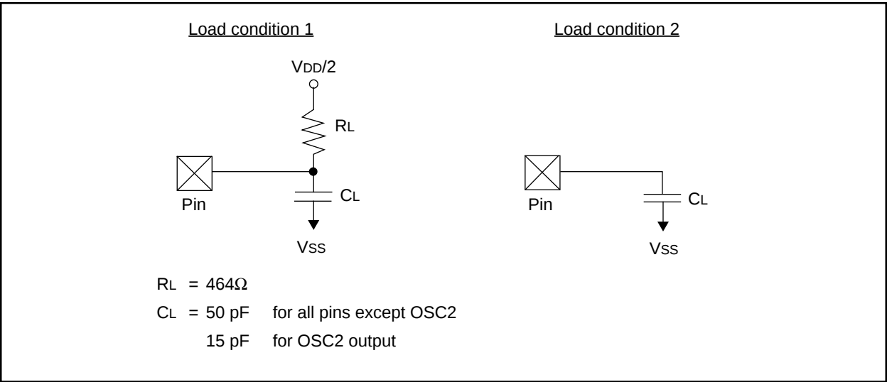
FIGURE 12-7: LOAD CONDITIONS
