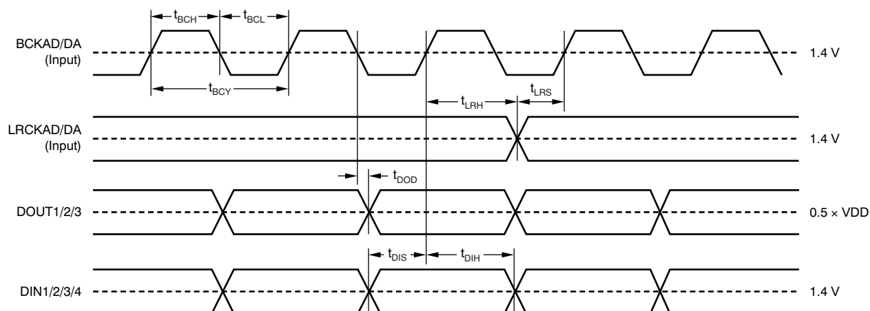
Figure 42. Audio Interface Timing Requirements for Left-Justified, Right-Justified, and I²S Data Formats (Slave Mode)
