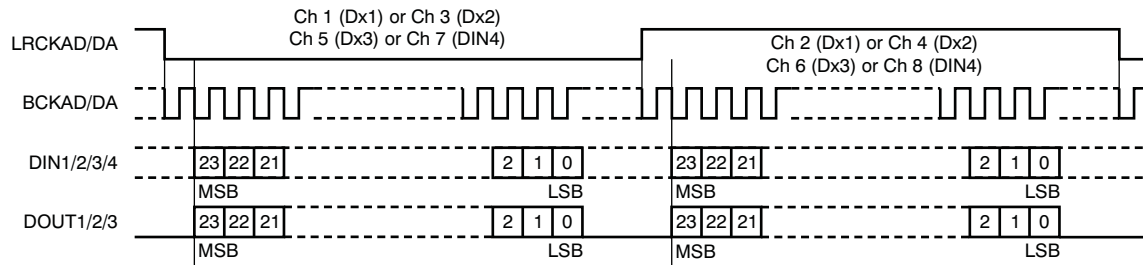
Figure 35. Audio Data Format: 24-Bit I 2 S
