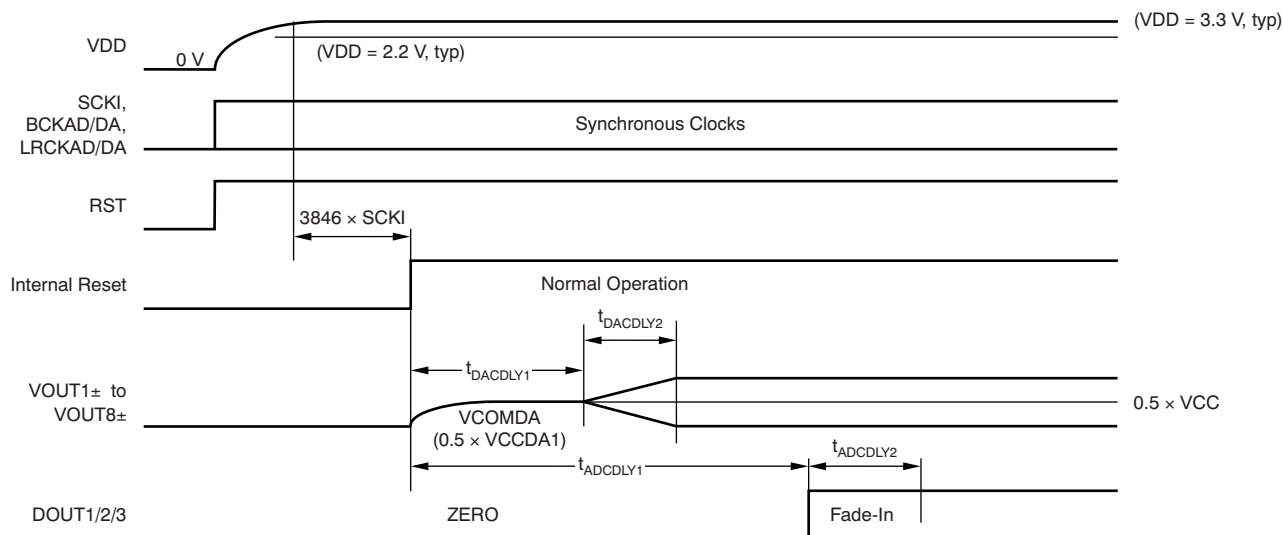
Figure 33. Power-On-Reset Timing Requirements
