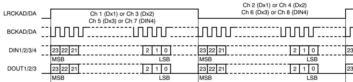
Figure 36. Audio Data Format: 24-Bit Left-Justified
