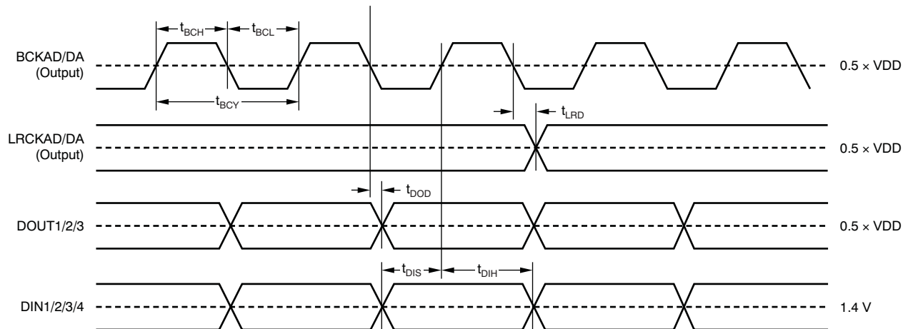
Figure 43. Audio Interface Timing Requirements for Left-Justified, Right-Justified, and I²S Data Formats (Master Mode)
