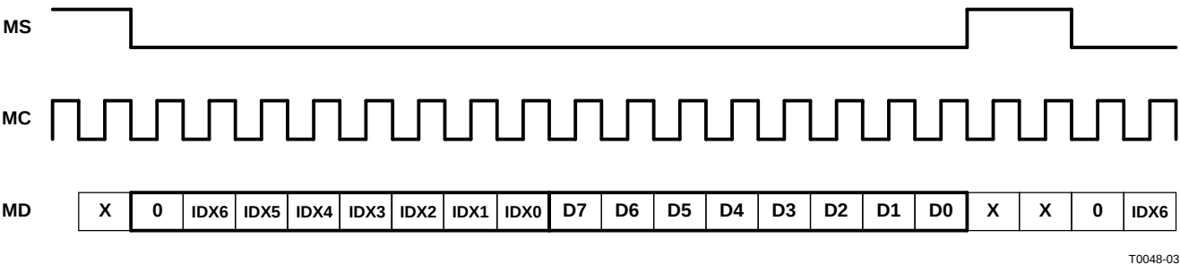
Figure 29. Serial Control Format
