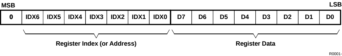
Figure 28. Control Data Word Format for MD
