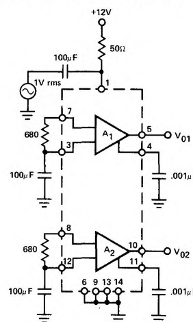
POWER SUPPLY REJECTION
