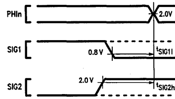
FIGURE 4-3. Timing Specification Standard (TTL Input Signals)
