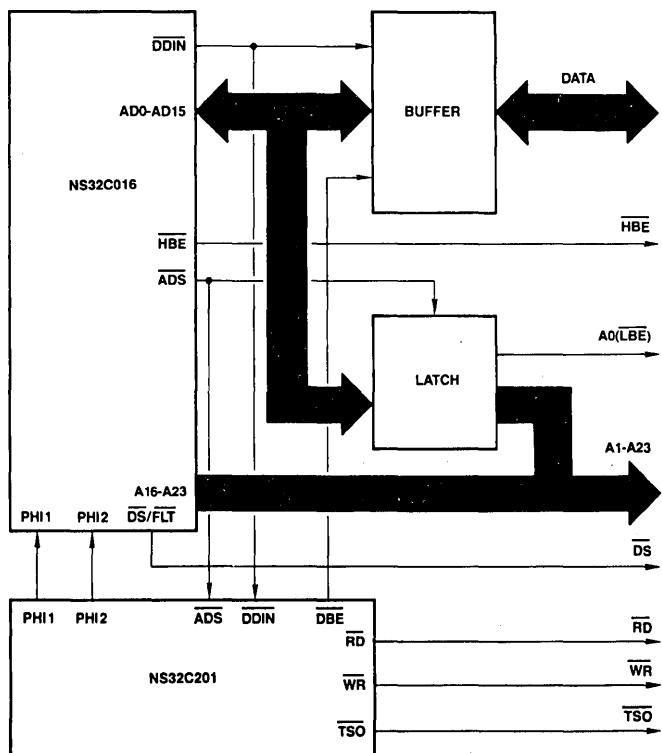
FIGURE 3-6. Bus Connections
