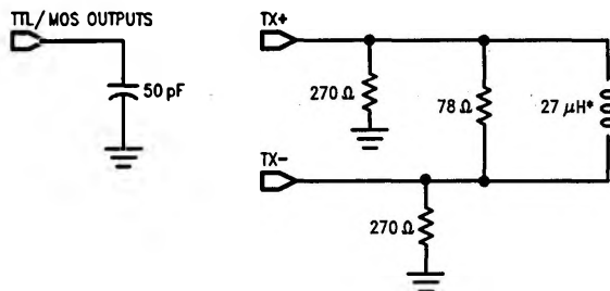
FIGURE 12. Test Loads
