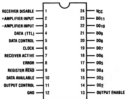
Dual-In-Line Package
