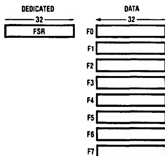
FIGURE 2-1. Register Set
