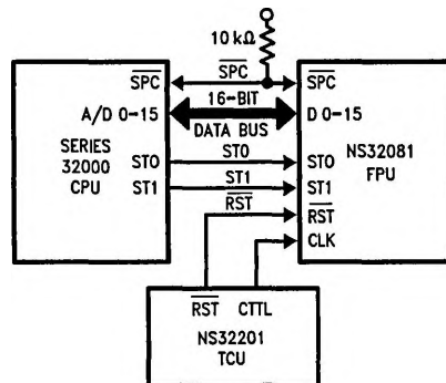
FIGURE 3-4. System Connection Diagram
