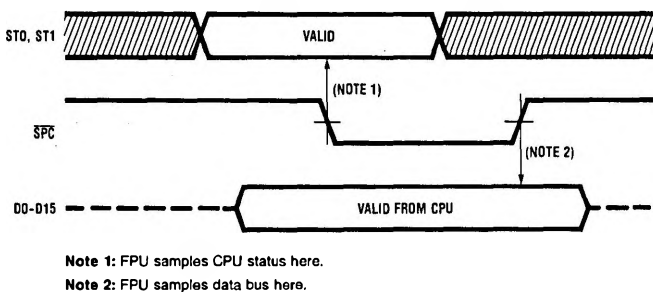
FIGURE 3-6. Slave Processor Write Cycle
