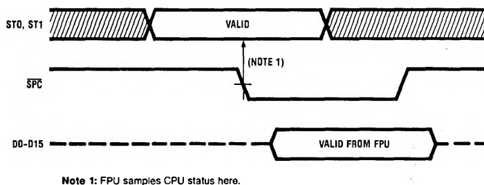
FIGURE 3-5. Slave Processor Read Cycle
