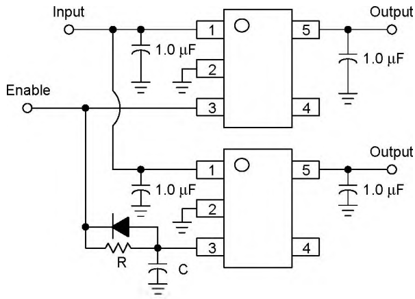
Figure 32. Delayed Turn-on
