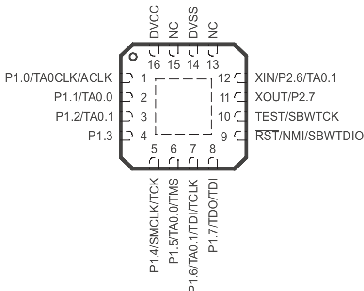
RSA PACKAGE (TOP VIEW)
