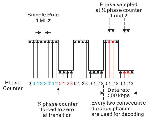
Figure 25-4. MFM Clock Synchronization
