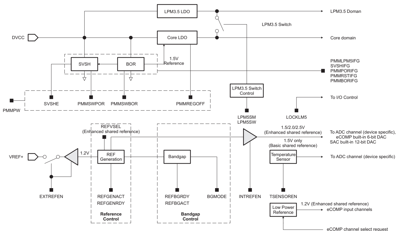
Figure 2-1. PMM Block Diagram
