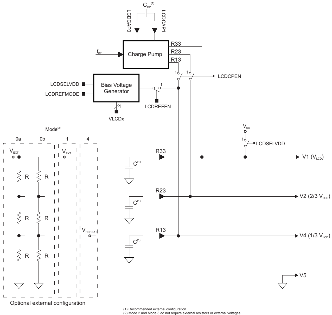
Figure 17-7. Bias Generation
