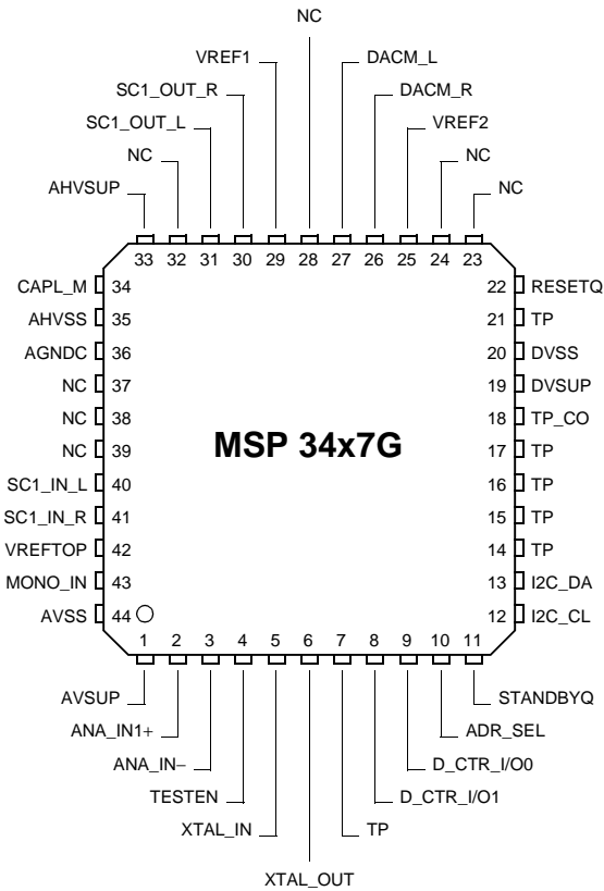
Fig. 4–4: PMQFP44 package
