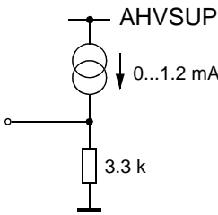
Fig. 4-15: Output Pins: DACM_R/L
