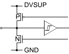
Fig. 4-13: Input/Output Pins: D_CTR_I/O_1, D_CTR_I/O_0
