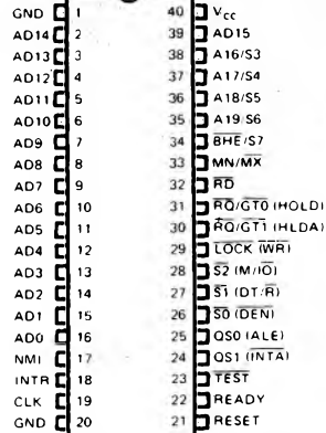
Fig. 2a MSM80C86ARS/MSM80C86A-2RS
