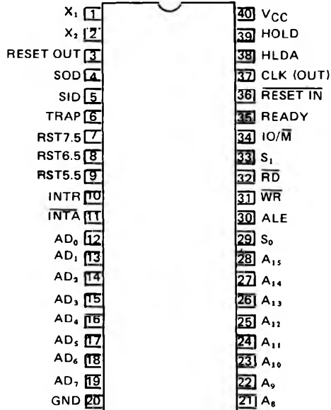
MSM80C85A-2 RS (Top View) 40 Lead Plastic DIP
