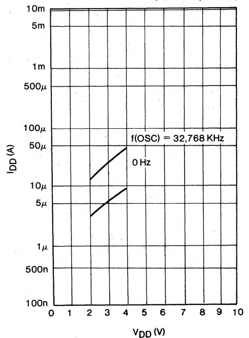
Current Consumption ( I_{DD} ) – Power Supply Voltage ( V_{DD} )
