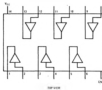
MM54C903/MM74C903 PMOS to TTL or CMOS Inverting Buffer
