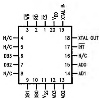
PCC Package
