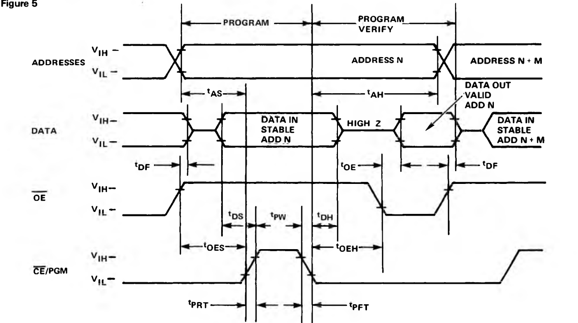
TIMING DIAGRAM (Program Mode) Figure 5
