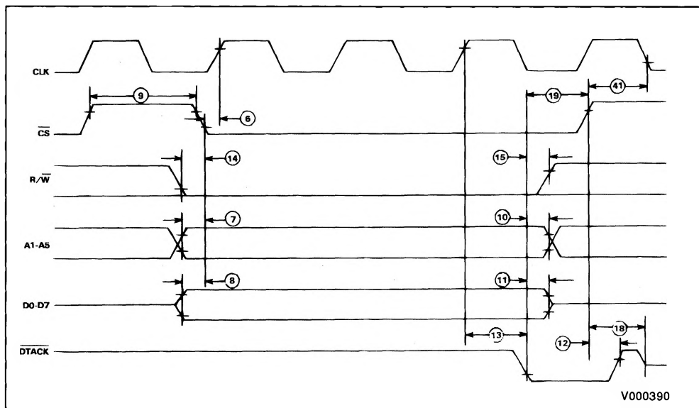
Figure 16 : Write Cycle.
