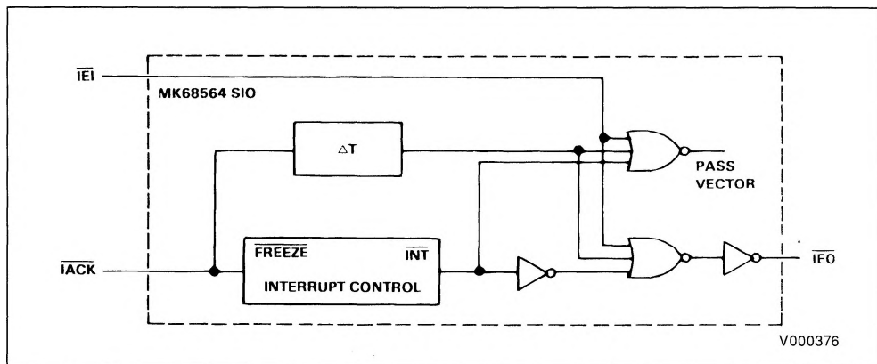
Figure 3 : Daisy Chaining.
