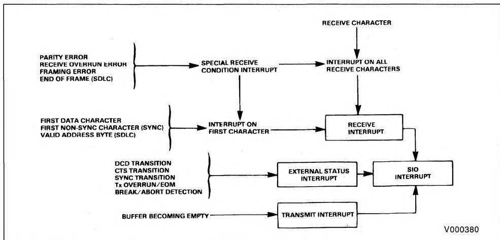
Figure 7 : Interrupt Structure.
