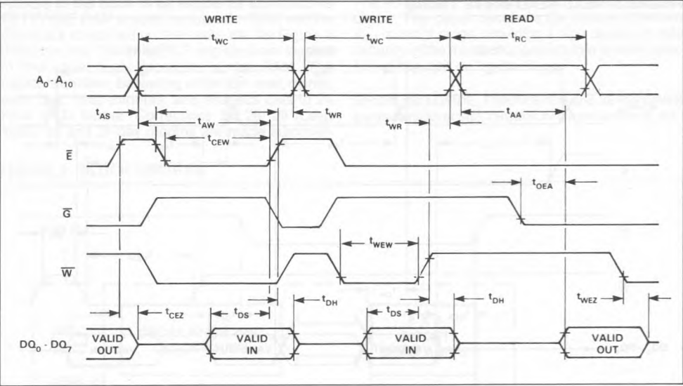
FIGURE 4. WRITE-WRITE-READ TIMING
