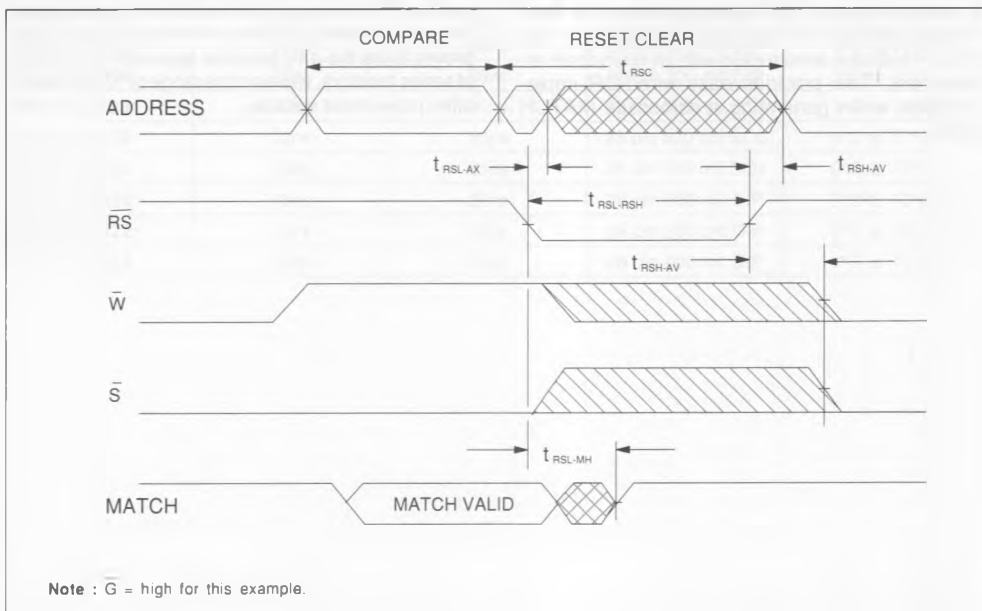
Figure 6 : Reset Timing.
