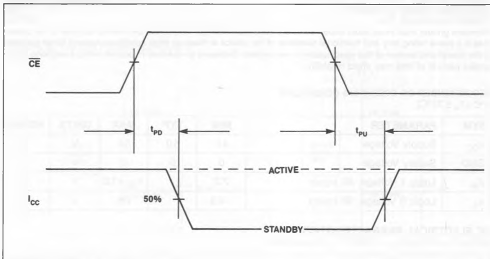
FIGURE 5. STANDBY MODE
