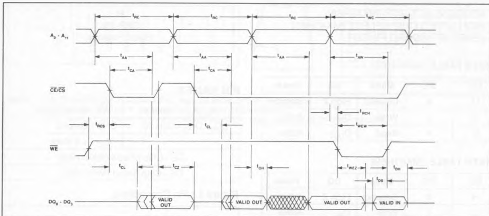
FIGURE 2. READ-READ-READ-WRITE TIMING
