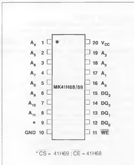
Figure 1 : Pin Connections.
