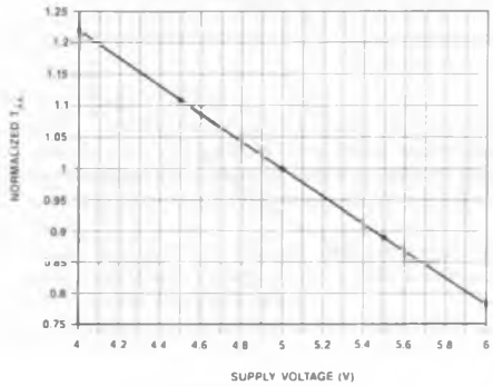
NORMALIZED ACCESS TIME VS SUPPLY VOLTAGE T_A=25^{\circ}C
