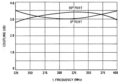
FIGURE 3 – COUPLING versus FREQUENCY
