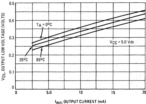
FIGURE 11 – TYPICAL OUTPUT LOW VOLTAGE versus OUTPUT CURRENT
