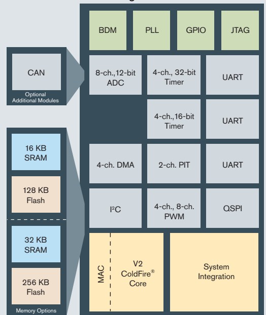
MCF5211/12/13 Block Diagram
