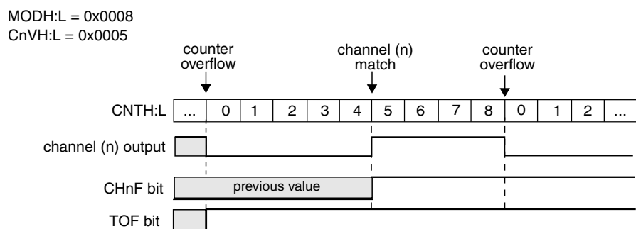
Figure 12-13. EPWM signal with ELSnB:ELSnA = X:1
