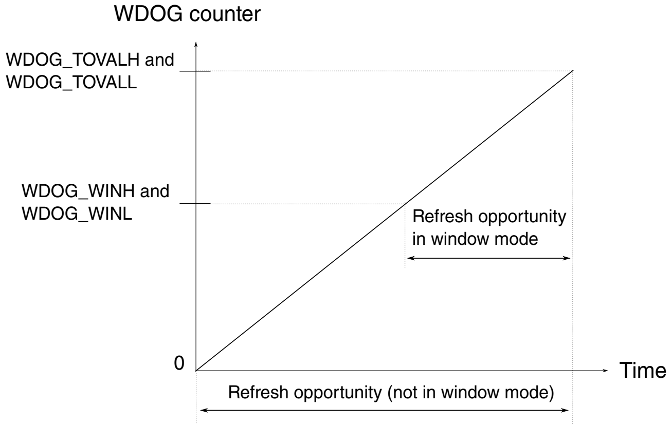
Figure 17-2. Refresh opportunity for the Watchdog counter
