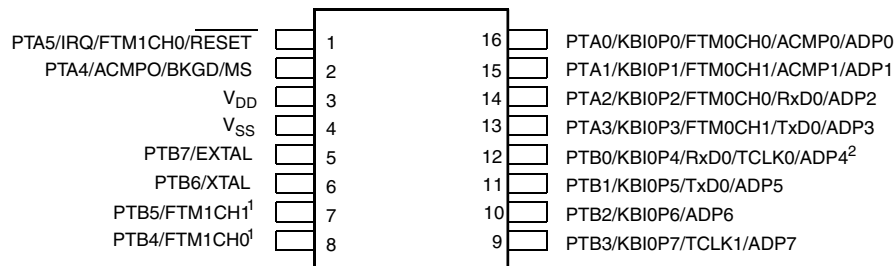
Figure 2-1. MC9S08PA4 20-pin SOIC/TSSOP packages
