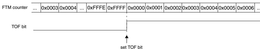
Figure 12-6. Example when the FTM counter is a free running
