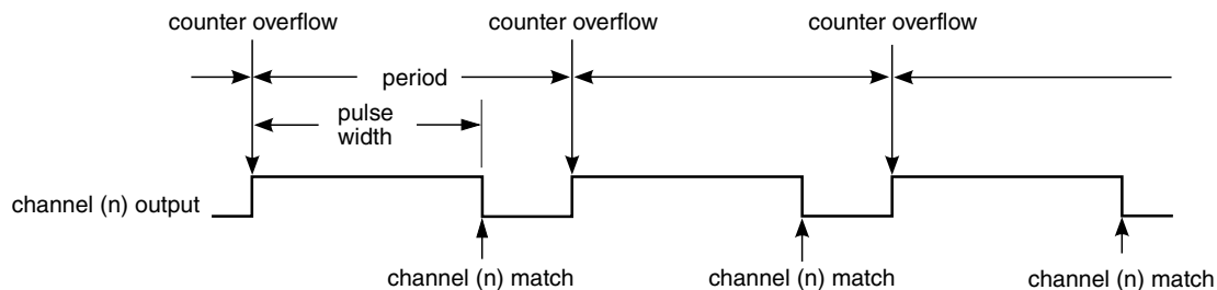
Figure 12-11. EPWM period and pulse width with \text{ELSnB:ELSnA} = 1:0
