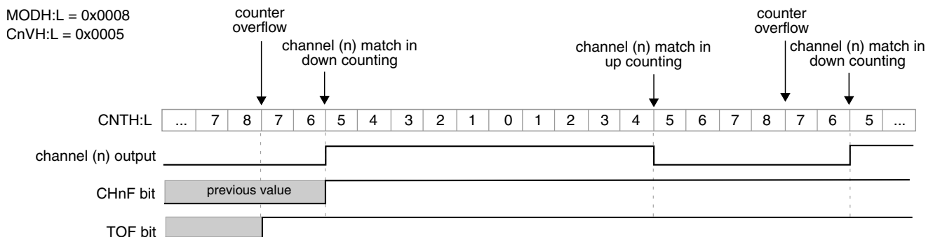
Figure 12-15. CPWM signal with ELSnB:ELSnA = 1:0
