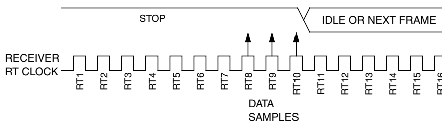
Figure 14-5. Fast data
