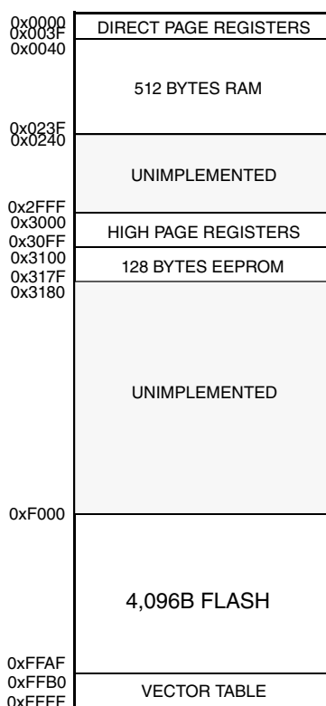
Figure 4-1. Memory map
