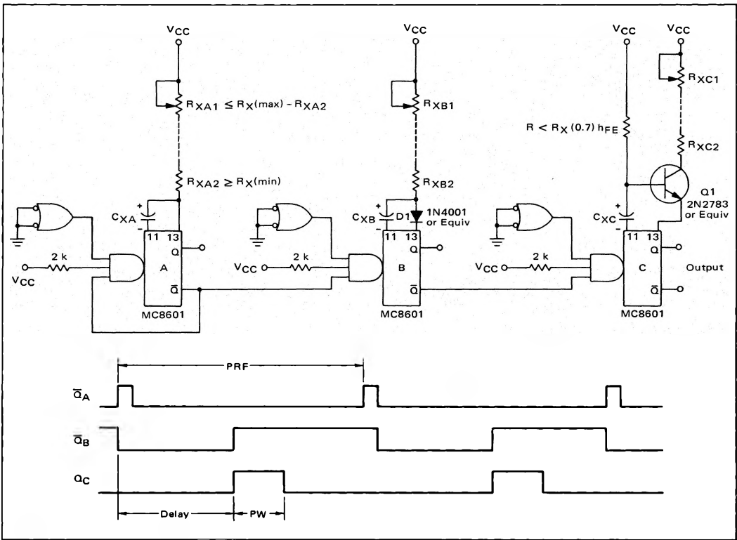
FIGURE 16 – PULSE GENERATOR
