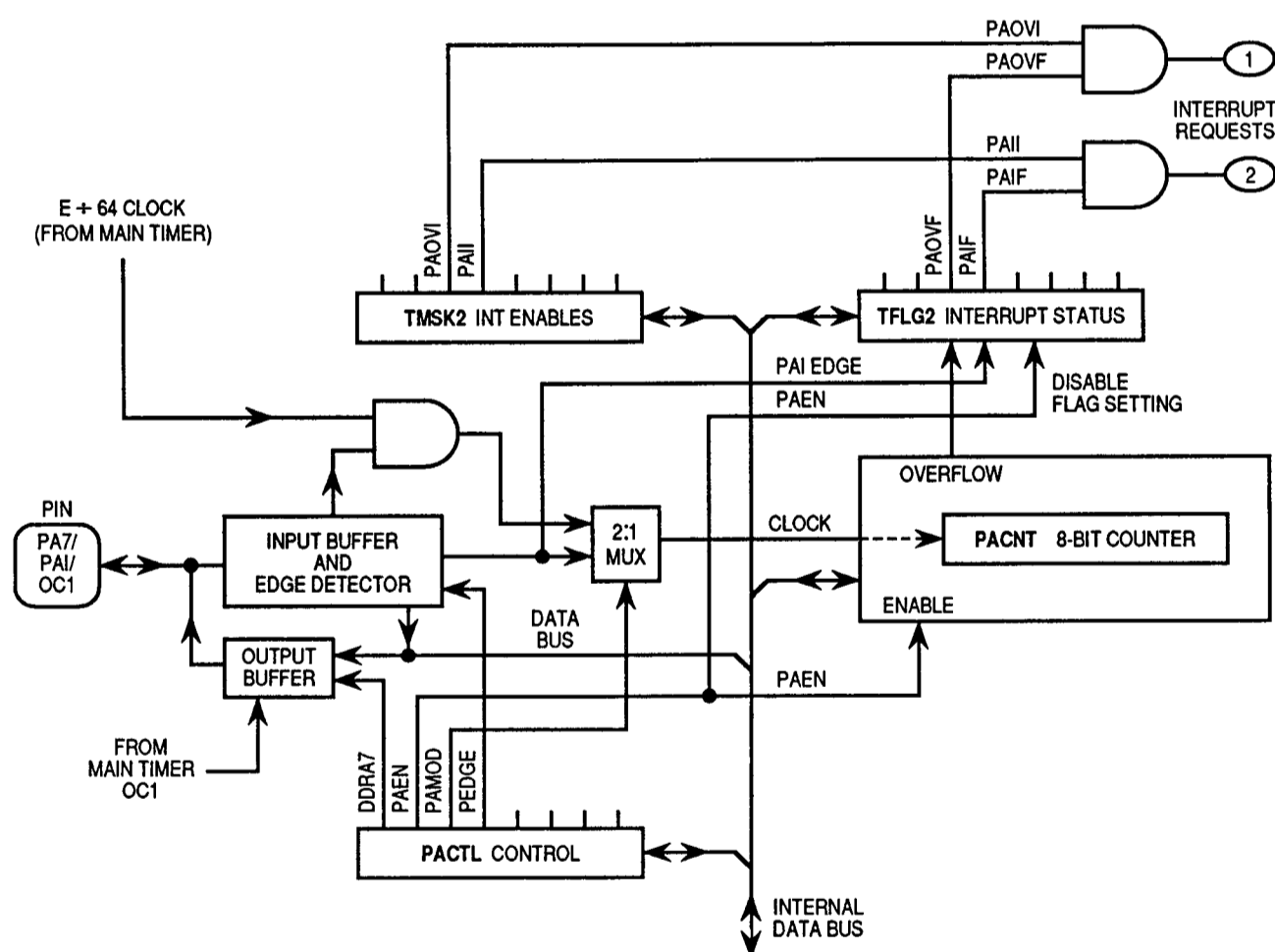
Figure 9–3. Pulse Accumulator
