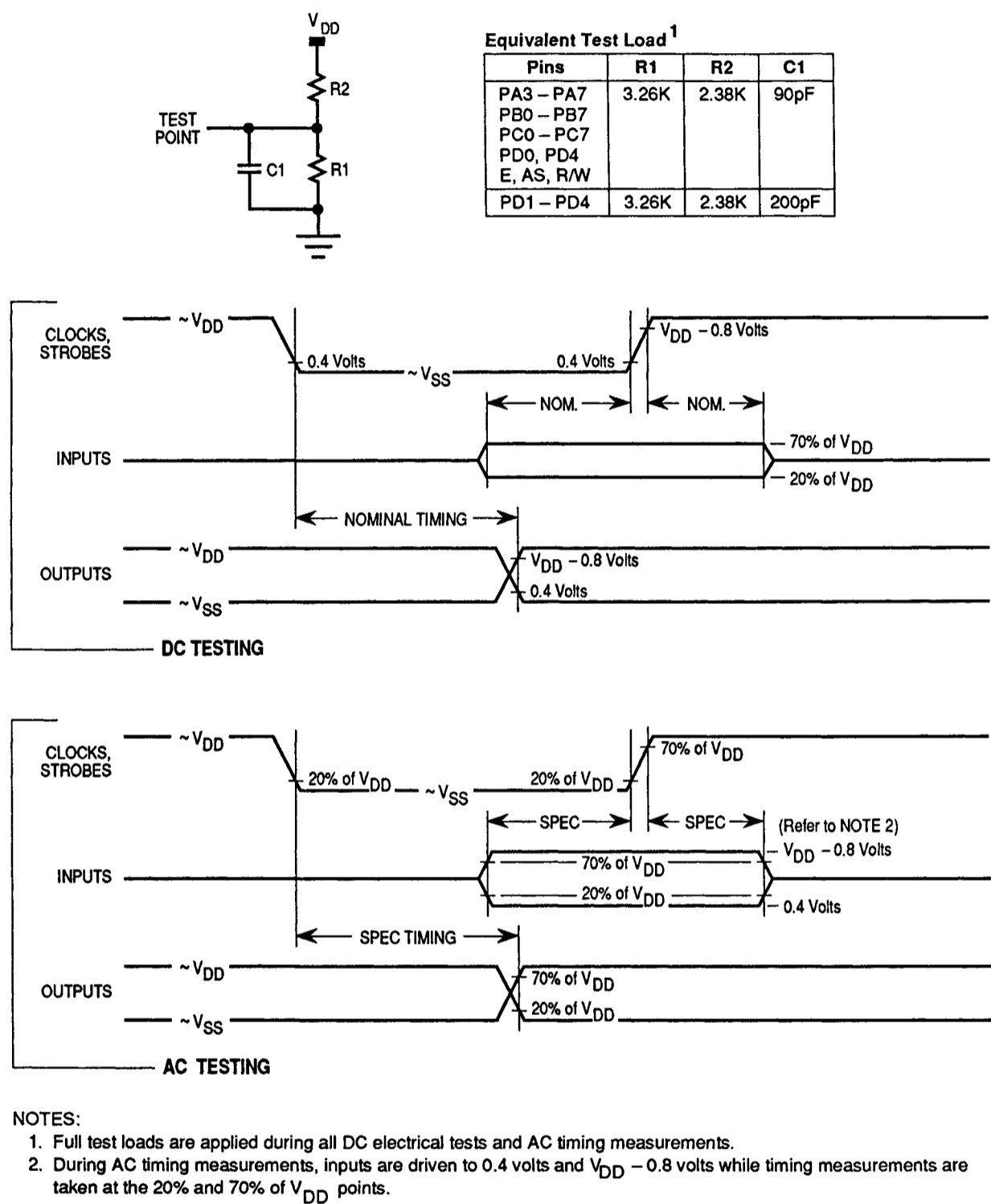
Figure A–1. Test Methods
