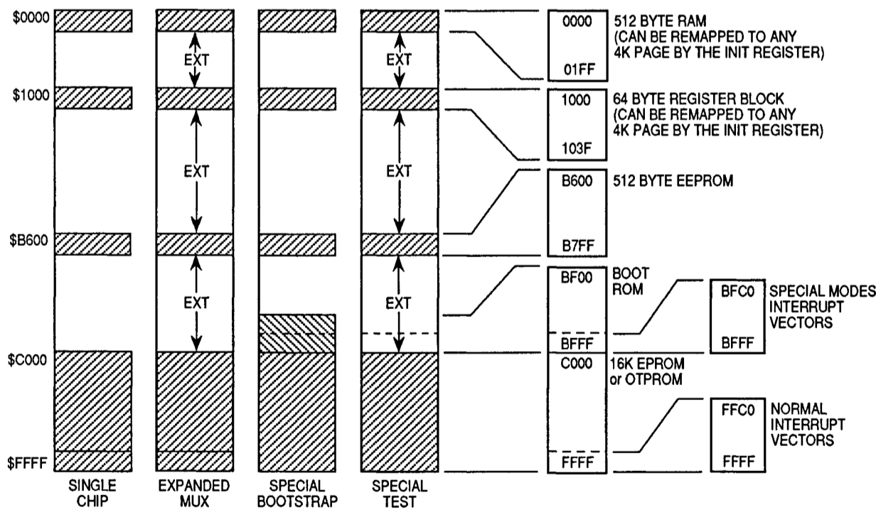
Figure 4–2. Memory Map
