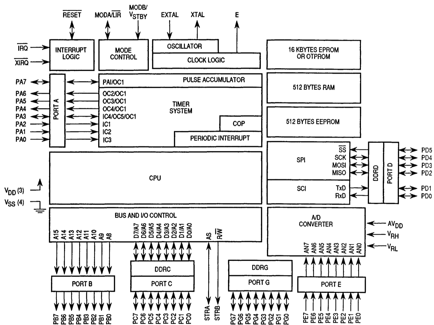
Figure 1–1. MC68HC711L6 Block Diagram
