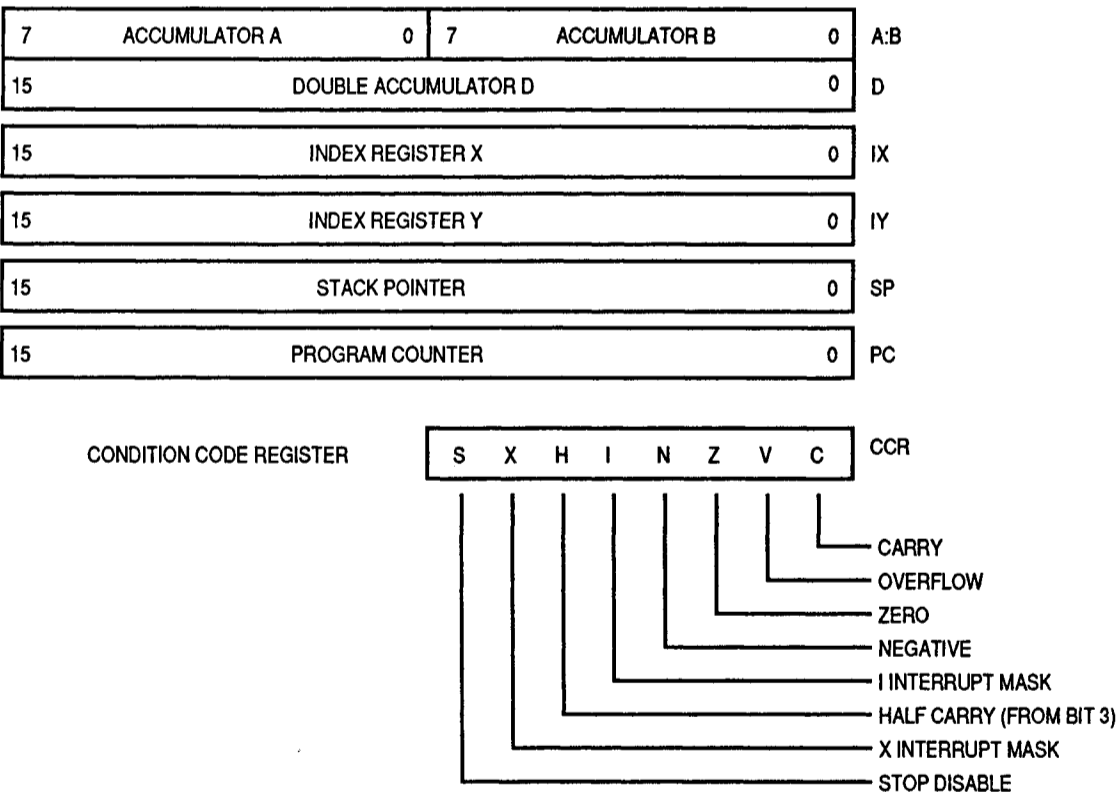
Figure 3-1. Programming Model
