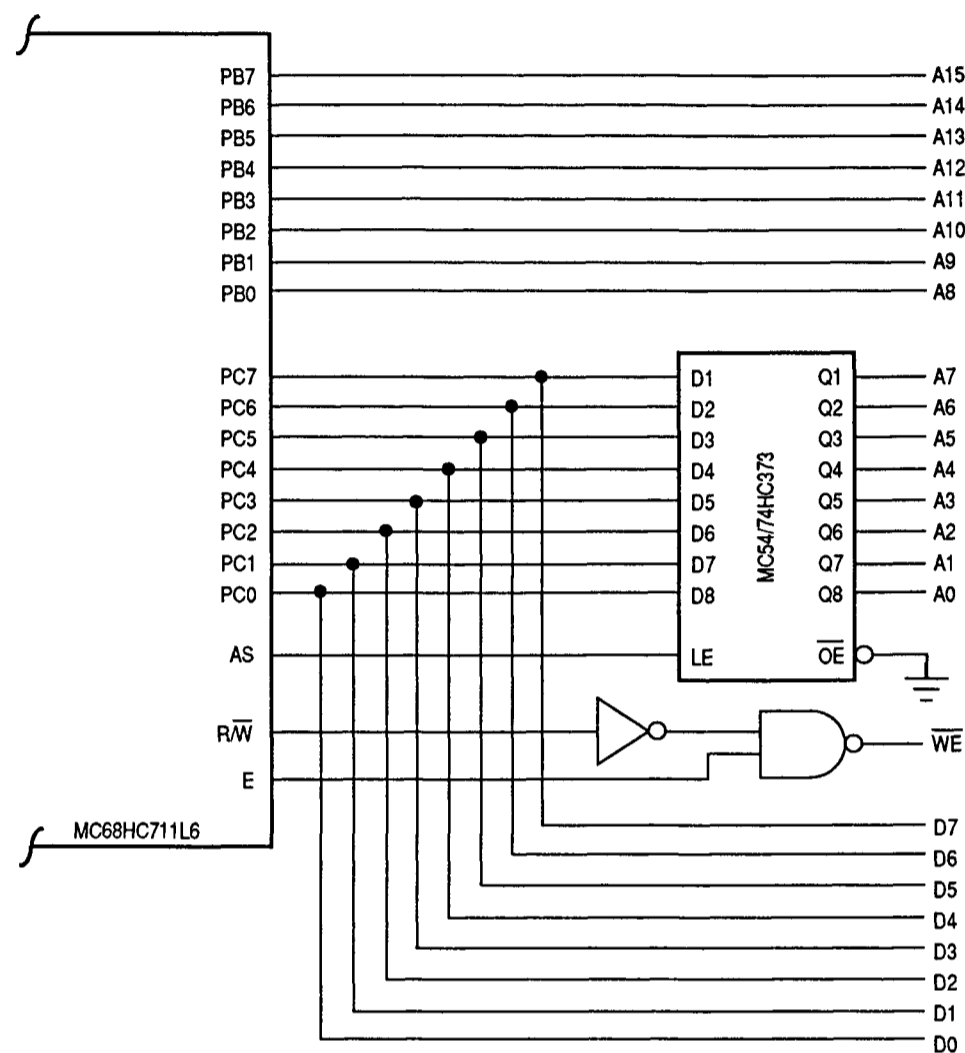
Figure 4-1. Address/Data Demultiplexing
