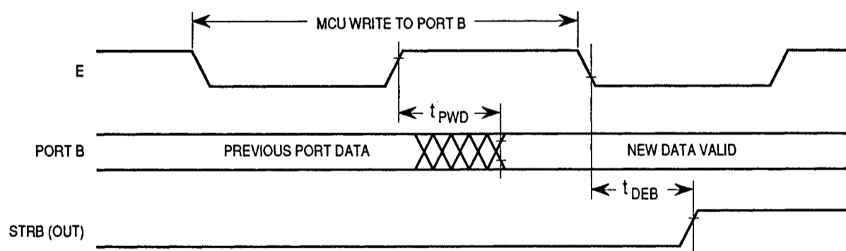
Figure A-9. Simple Output Strobe Timing Diagram
