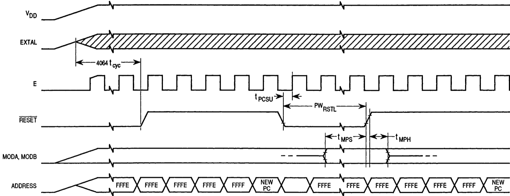
Figure A-3. POR and External Reset Timing Diagram
