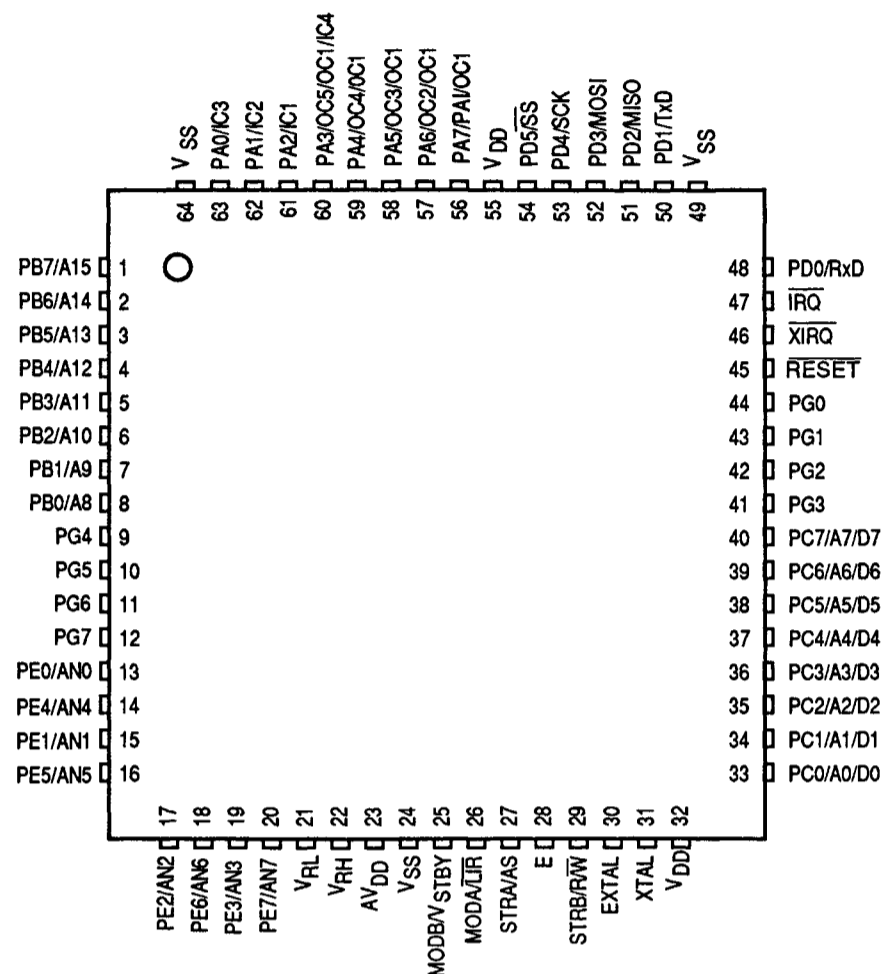
Figure 2-2. Pin Assignments for 64-Pin QFP
