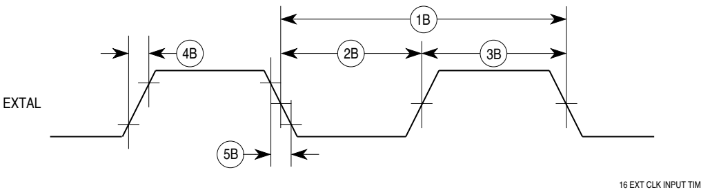
Figure 22 External Clock Input Timing Diagram
