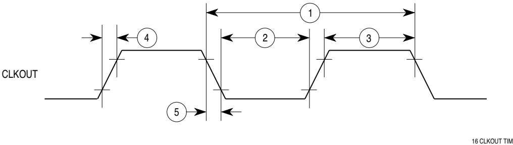
Figure 21 CLKOUT Output Timing Diagram
