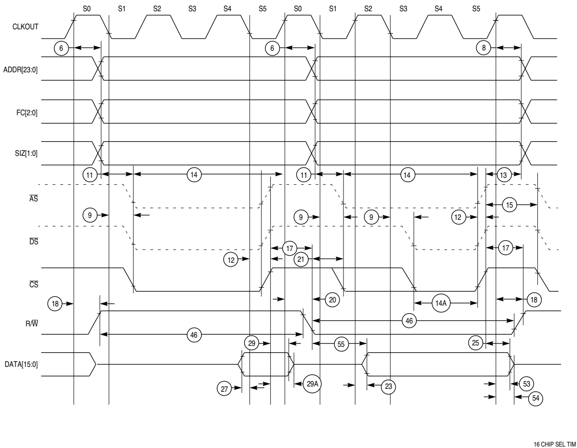
Figure A-11 Chip-Select Timing Diagram
