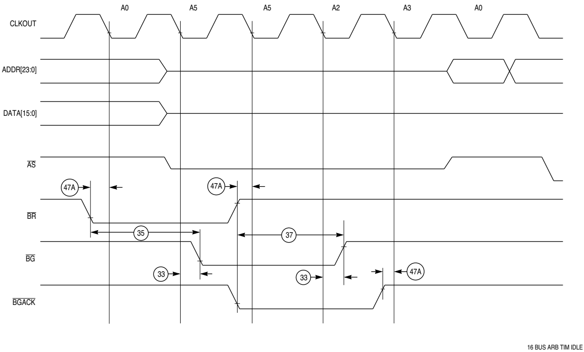
Figure 29 Bus Arbitration Timing Diagram — Idle Bus Case
