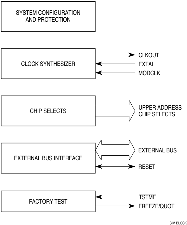
Figure 8 SIM Block Diagram
