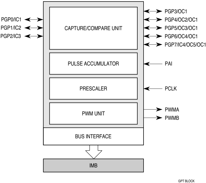
Figure 17 GPT Block Diagram
