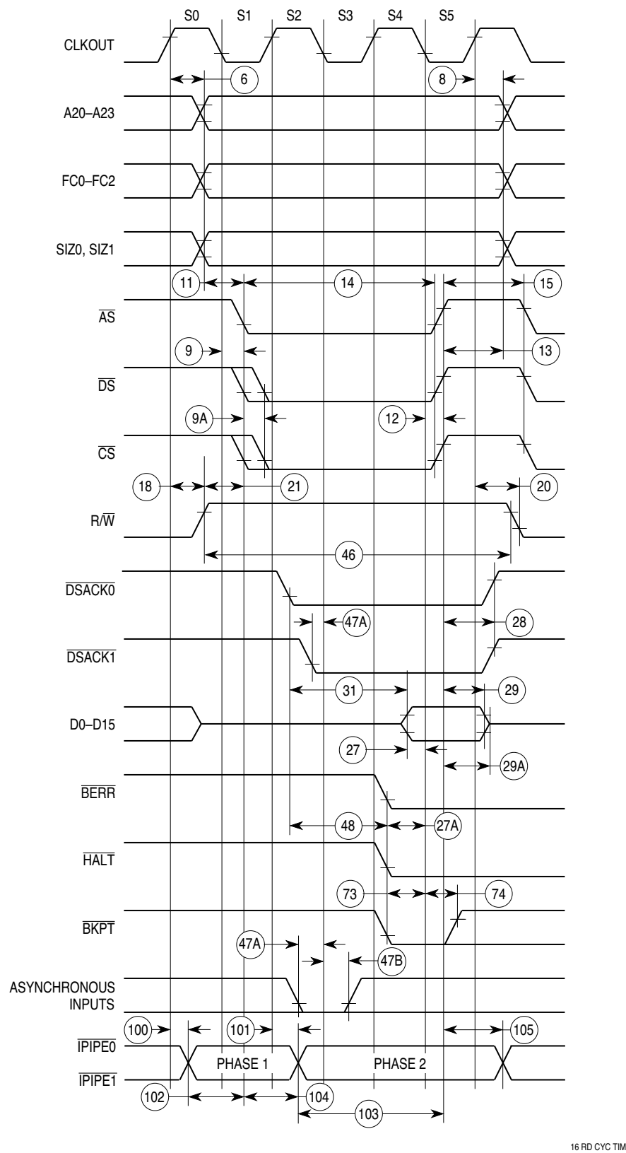
Figure 24 Read Cycle Timing Diagram
