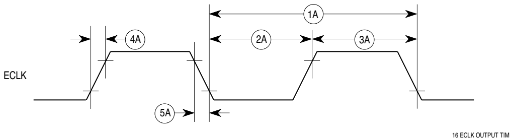
Figure 23 ECLK Output Timing Diagram
