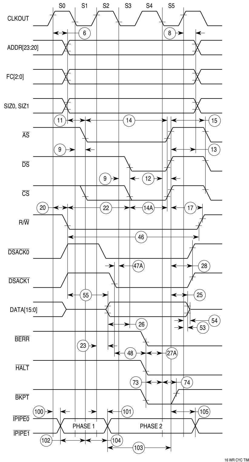
Figure 25 Write Cycle Timing Diagram
