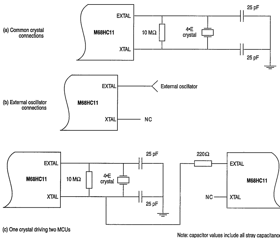
Figure 2-3 Oscillator connections (VDDSYN = 0, PLL disabled)
