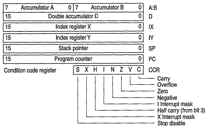
Figure 3-1 Programming model
