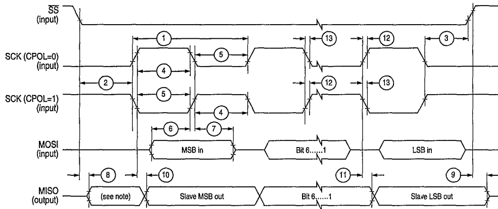
Figure A-11 SPI slave timing (CPHA = 0)
