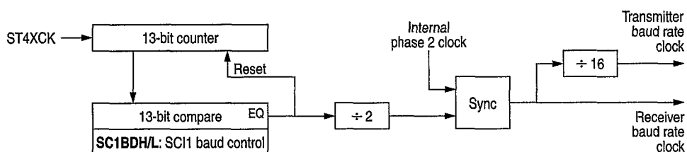
Figure 7-1 SCI1 baud rate generator circuit diagram
