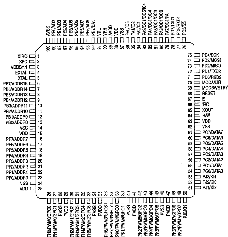
Figure 2-1 100-pin TQFP
