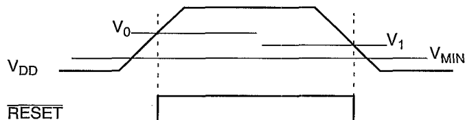
Figure 5-1 Power on reset
