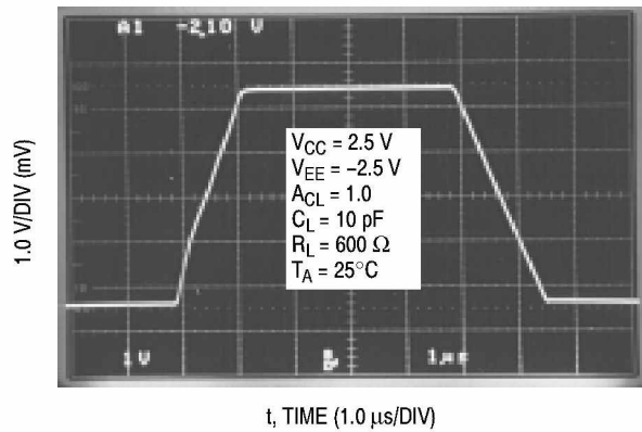
Figure 8. Slew Rate
