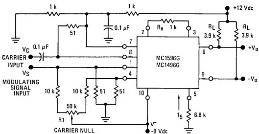
FIGURE 27 – BALANCED MODULATOR-DEMODULATOR
