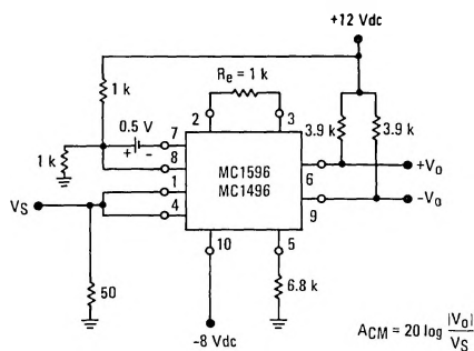
FIGURE 11 – COMMON-MODE GAIN
