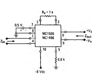
FIGURE 8 – INPUT-OUTPUT IMPEDANCE
