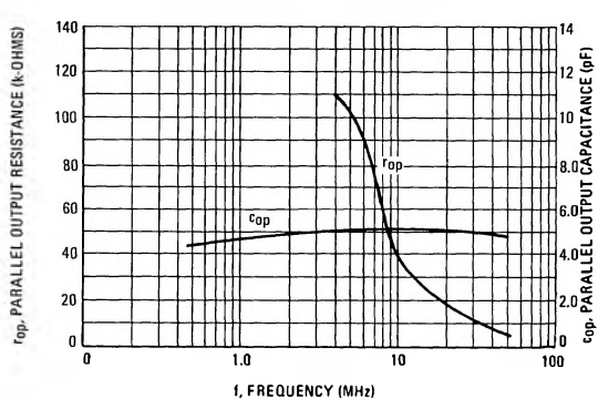
FIGURE 16 – SINGLE-ENDED OUTPUT IMPEDANCE versus FREQUENCY
