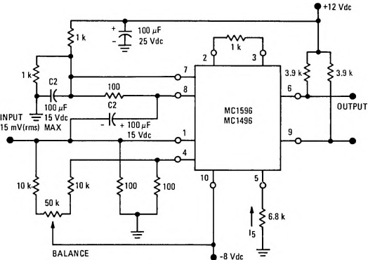
FIGURE 31 – LOW-FREQUENCY DOUBLER
