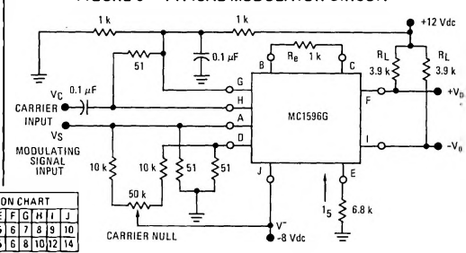
FIGURE 6 – TYPICAL MODULATOR CIRCUIT
