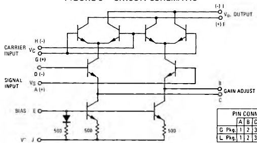
FIGURE 5 – CIRCUIT SCHEMATIC
