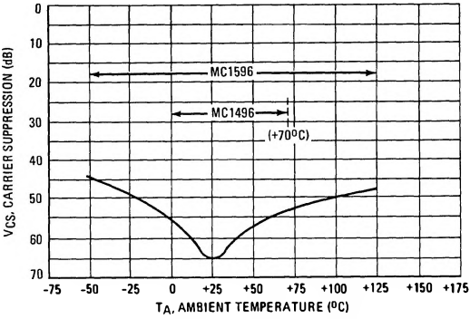
FIGURE 18 – CARRIER SUPPRESSION versus TEMPERATURE
