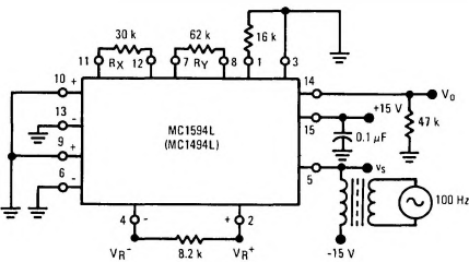
FIGURE 7 – POWER-SUPPLY SENSITIVITY
