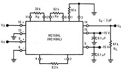
FIGURE 7 – POWER-SUPPLY SENSITIVITY
