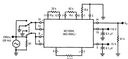
FIGURE 6 – COMMON-MODE
