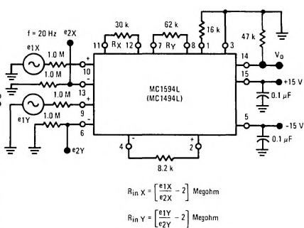
FIGURE 2 – INPUT RESISTANCE
