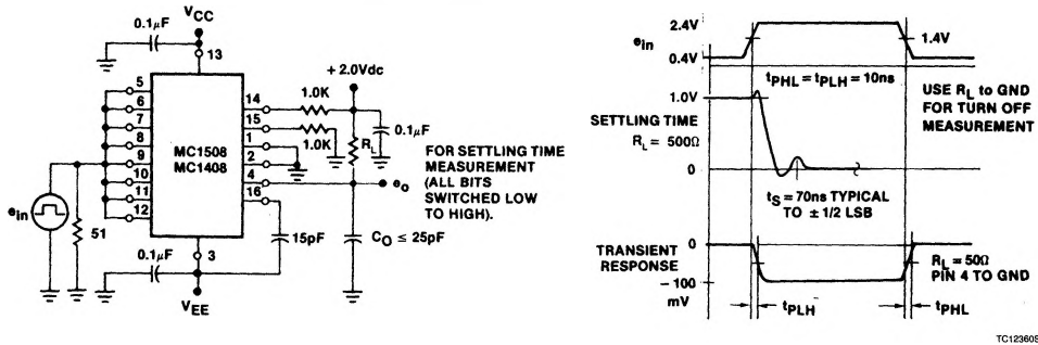
Figure 4. Transient Response and Settling Time
