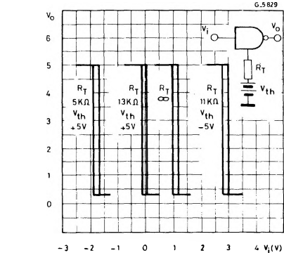
Figure 8 : MC1489 Input Threshold Adjustment.
