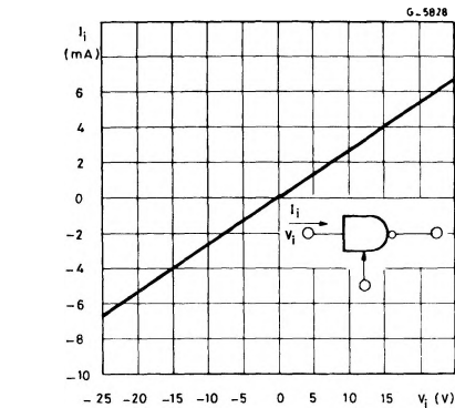
Figure 7 : Input Current.
