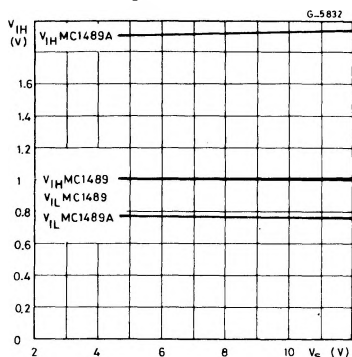
Figure 11 : Input Threshold vs. Power-Supply Voltage.
