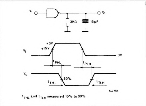
Figure 6 : Switching Response.
