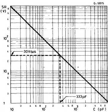
Figure 12 : Slew Rate vs. Capacitance for I sc = 10mA.
