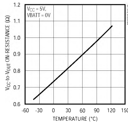
V_{CC} to V_{OUT} ON-RESISTANCE vs. TEMPERATURE
