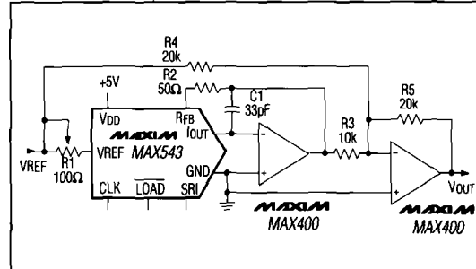
Figure 4. Bipolar Operation
