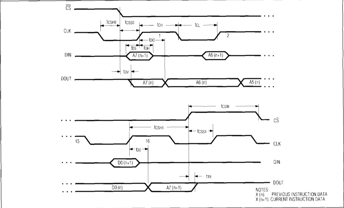
Figure 5. Timing Diagram
