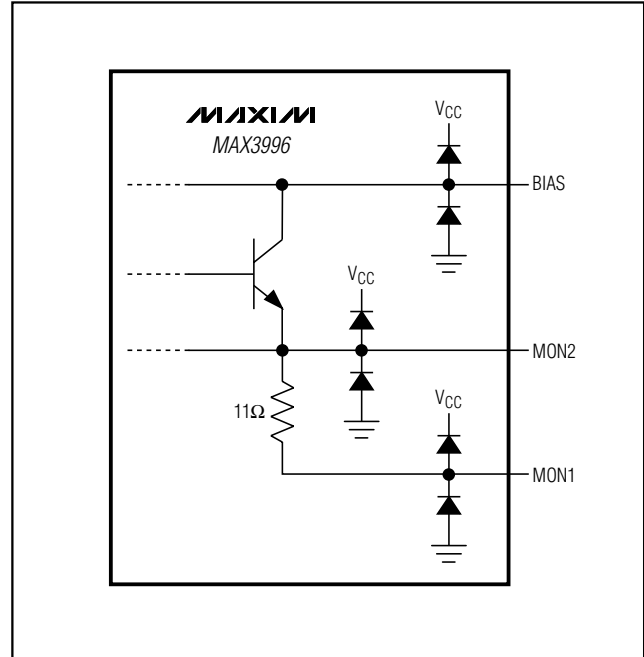
Figure 17. BIAS Output
