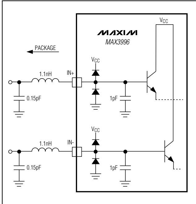
Figure 16. Data Inputs
