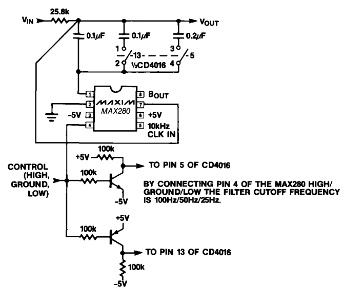
100Hz, 50Hz, 25Hz 5th Order DC Accurate LP Filter
