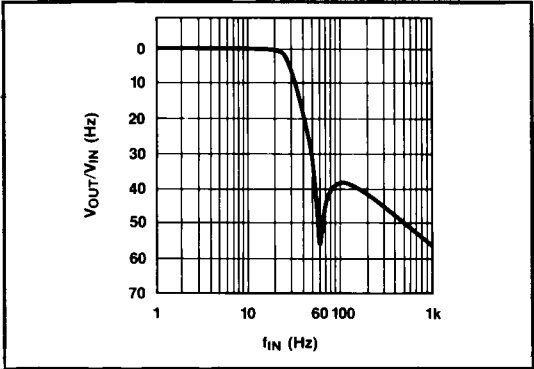
Figure 8D. Amplitude Response of the Filter
