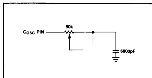
Figure 2. External Oscillator Trim
