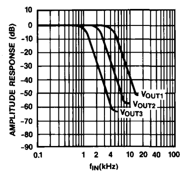
Amplitude Response for the Octave Tuning Circuit
