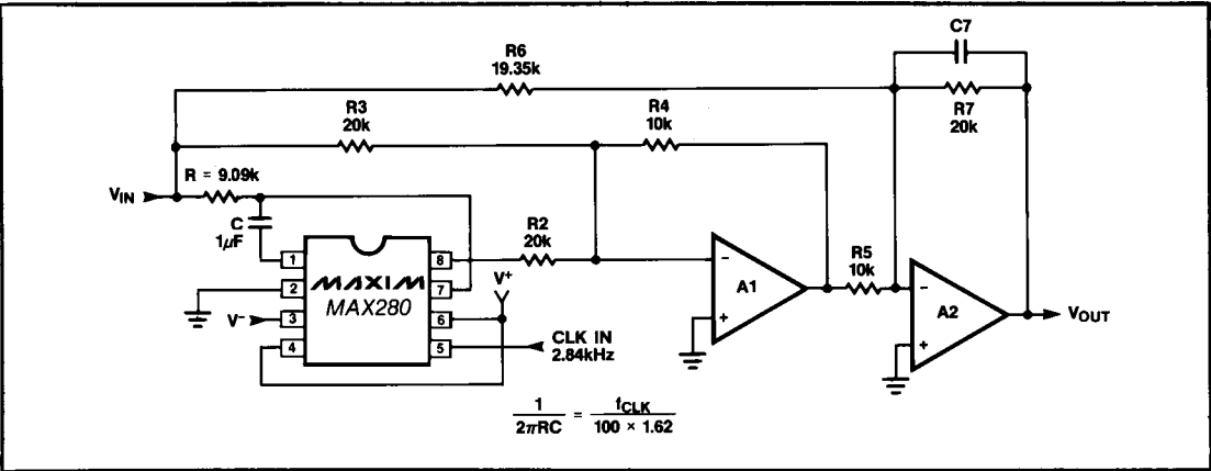
Figure 8C. A Lowpass Filter with a 60Hz Notch
