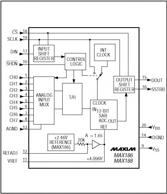
Figure 3. Block Diagram
