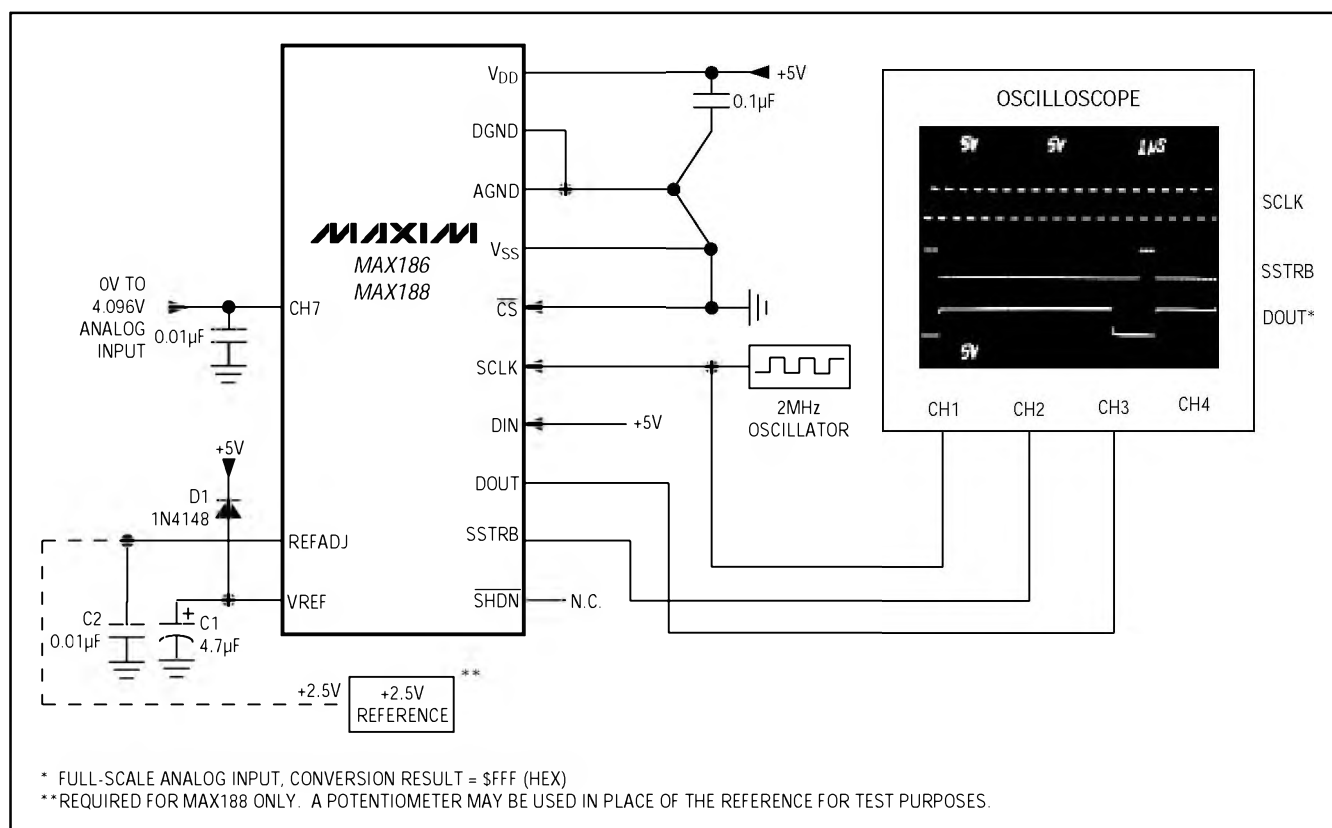
Figure 5. Quick-Look Circuit
