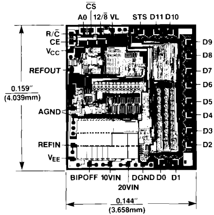
Chip Topography
