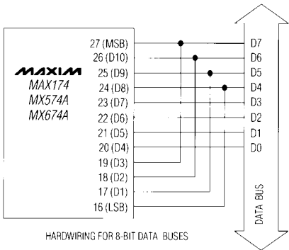
HARDWIRING FOR 8-BIT DATA BUSES
