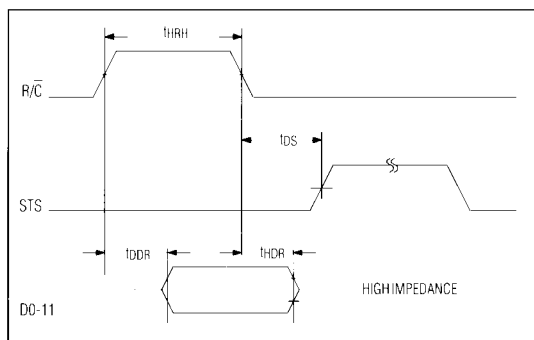
Figure 7. High Pulse for R/C in Stand-Alone Mode
