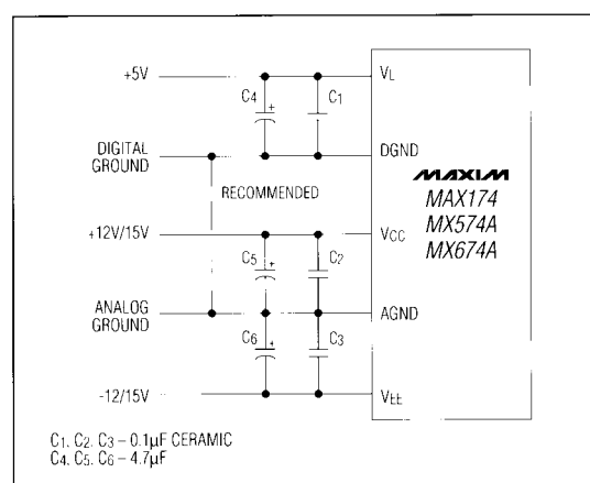
Figure 9. Power-Supply Bypassing
