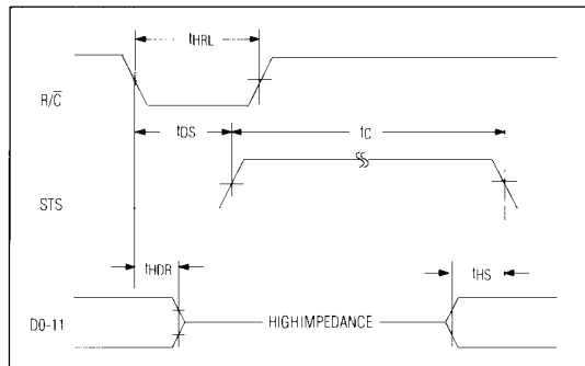
Figure 6. Low Pulse for R/C in Stand-Alone Mode
