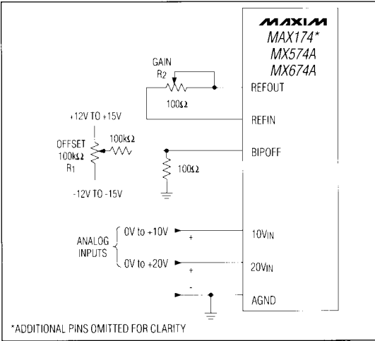
Figure 13. Unipolar Input Connections
