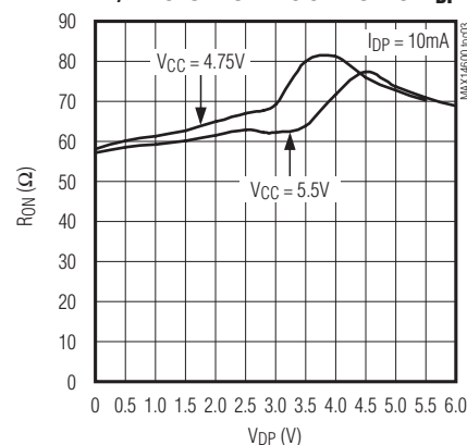
DP/DM SHORT ON-RESISTANCE vs. VDP
