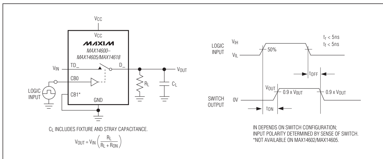
Figure 1. Switching Time
