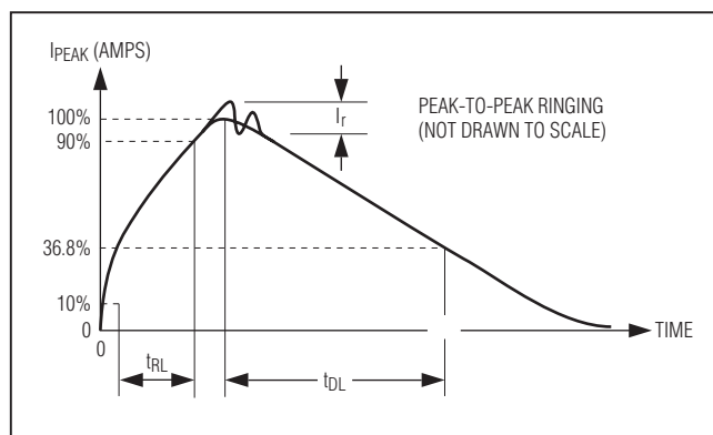
Figure 7b. Human Body Current Waveform
