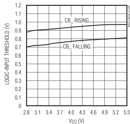
LOGIC-INPUT THRESHOLD vs. SUPPLY VOLTAGE
