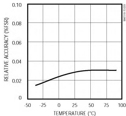
MAX1111 RELATIVE ACCURACY vs. TEMPERATURE
