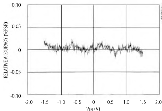
MAX1111 RELATIVE ACCURACY ( -0.667V_{REF} < V_{IN} < 0.667V_{REF} )
