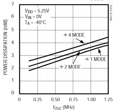
MAX1111 POWER DISSIPATION vs. OVERSAMPLING FREQUENCY ( f_{OSC} )
