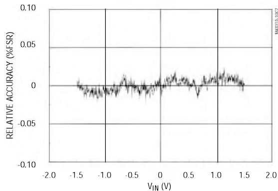
MAX1111 RELATIVE ACCURACY ( -V_{REF} < V_{IN} < V_{REF} )
