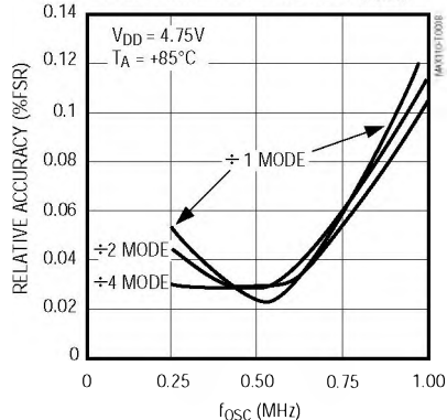
MAX1111 RELATIVE ACCURACY vs. OVERSAMPLING FREQUENCY ( f_{OSC} )
